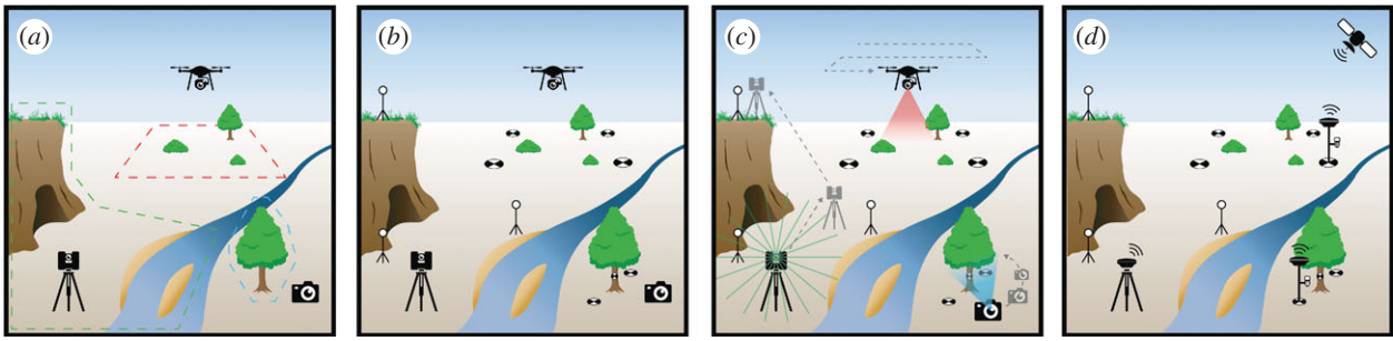
Figure 2. Major steps for capturing data with terrestrial laser scanning and structure-from-motion using handheld and drone-mounted cameras. (a) Identify features of interest and estimate scanning positions or camera angles. (b) Set out reference targets for terrestrial laser scanning, or ground control points, check points and scaling objects for structure-from-motion. For laser scanning, targets are used to align data from different stations, although scene geometry can sometimes be used for alignment instead of, or in addition to targets. For structure-from-motion, reference points are used for aligning images and constraining the modelling process, and for accuracy assessment and scaling. (c) Terrestrial laser scanning collects data from a number of discrete stations, to be combined during processing. For structure-from-motion, many overlapping photographs are taken, from which a 3D model is generated during processing. (d) Georeferencing, typically using a commercial-grade global navigation satellite system, is required to position the resulting 3D models in real-world space, and for scaling in large structure-from-motion models. (Online version in colour.)
