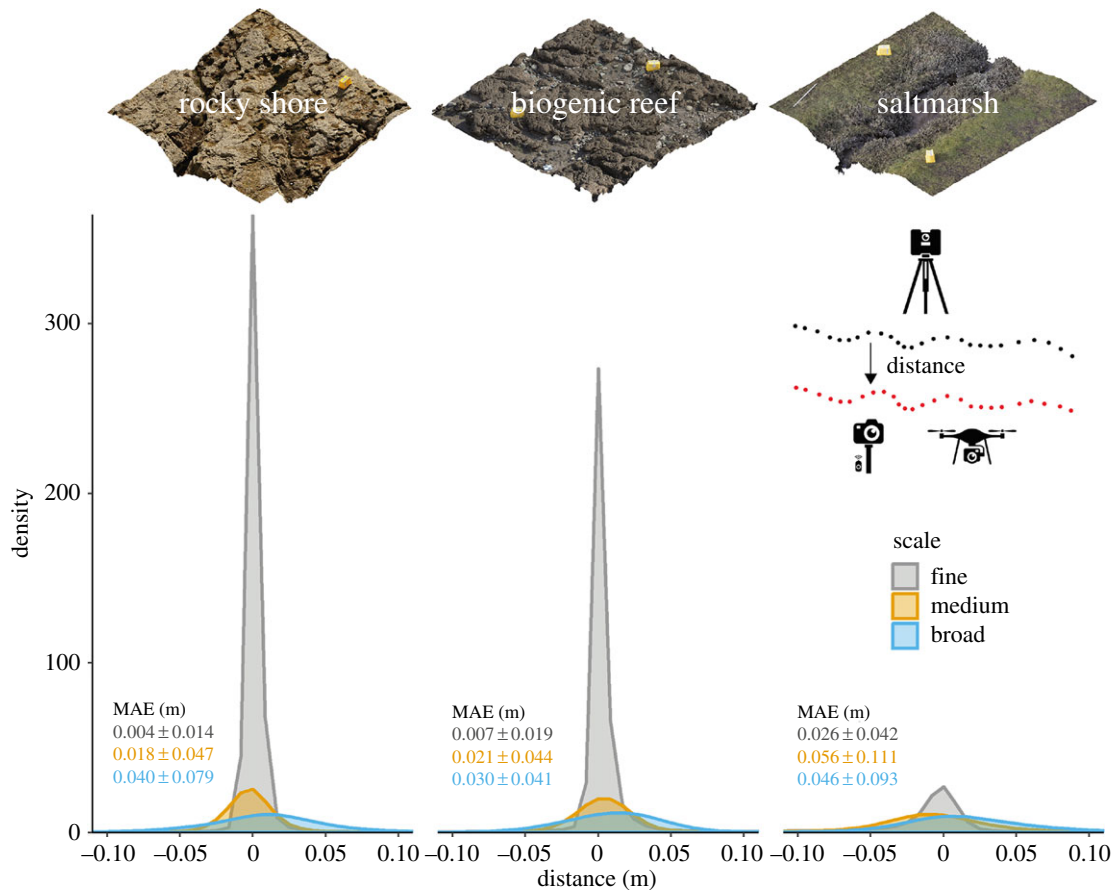
Figure 3. Accuracy of a structure-from-motion point cloud quantified as the point-by-point distance to a reference terrestrial laser scanning point cloud in three habitats (rocky shore, biogenic reef and saltmarsh) and at three scales (fine: 25 m 2 with less than 1 cm resolution, medium: 2500 m 2 with less than 2 cm resolution and broad: 2500 m 2 with 5 cm resolution). Distances were measured at 100 000 points and plotted as density curves, with the area under each curve being equal. Curve tails beyond 0 \pm 0.1 m are not shown. Mean absolute error (MAE) \pm 1 s.d. (m) distance is reported. (Online version in colour.)
